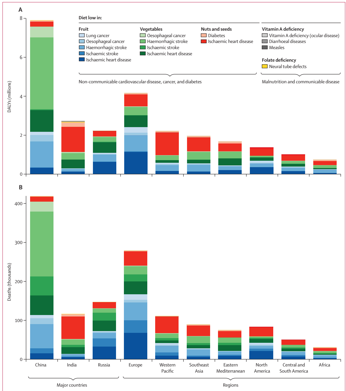
Figure 1: Burden of disease caused by pollinator removal, by cause and risk factor Additional yearly (A) DALYs lost and (B) deaths attributable to declines in pollinator-dependence foods and nutrients in countries with a significant health burden (China, India, and Russia) and elsewhere globally by region. DALY=disability-adjusted life-year.
