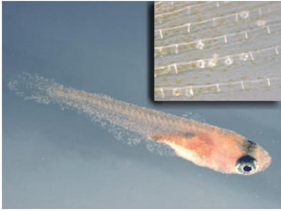
Figure 4. Medaka fish ( Oryzias latipes ) fry infested with the ectoparasite Cyclochaeta (= Trichodina ) domerguei (white circles in insert). Fish reared in a rice experimental paddy treated with imidacloprid were significantly more infested with these parasites compared to fish reared in non-treated paddies (after Sánchez-Bayo and Goka, 2005).
